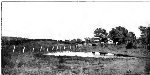
A. Morainic topography in northern part of area, with gentle swells and shallow basins.
